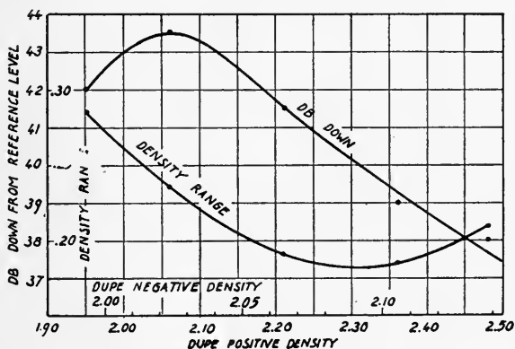
FIG. 7. Cross-modulation level as a function of combinations of dupe negative and dupe positive densities.
